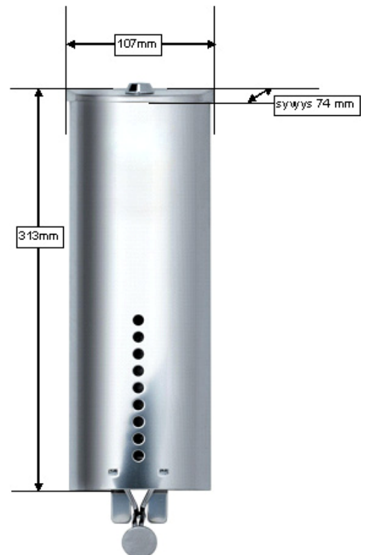
Dispenser-koteloteline 4065017
