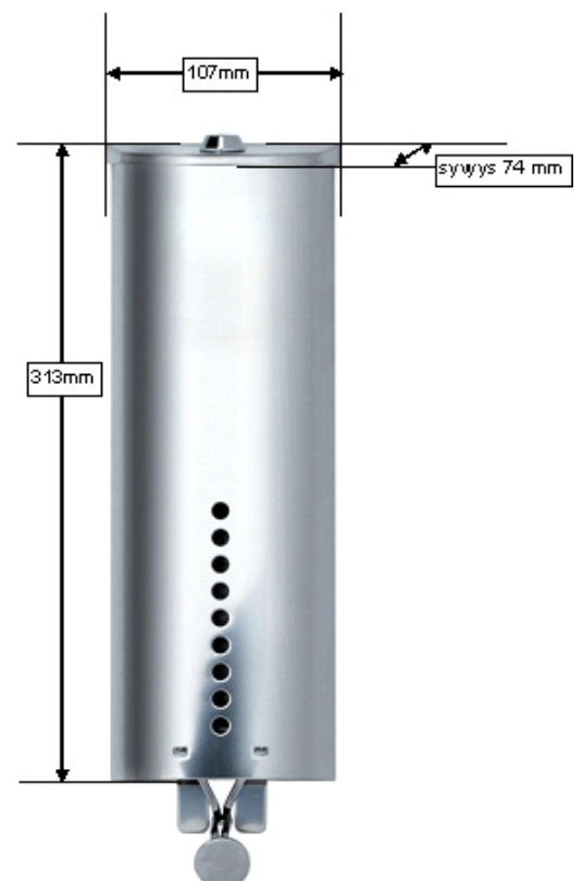
Dispenser-koteloteline 4065017
